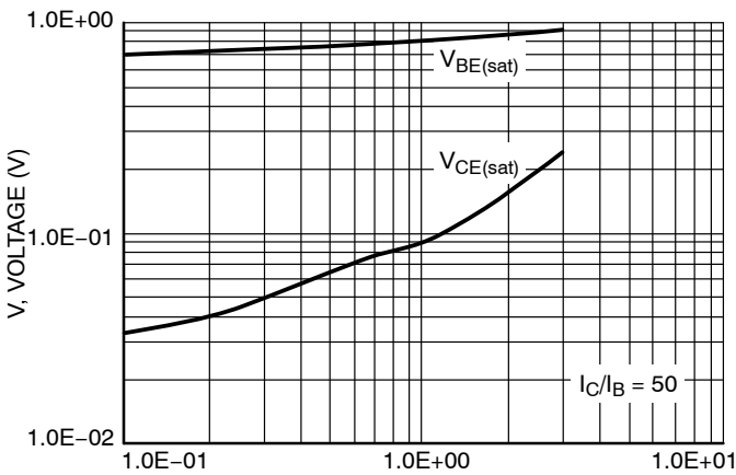
Figure 5. "ON" Voltages
